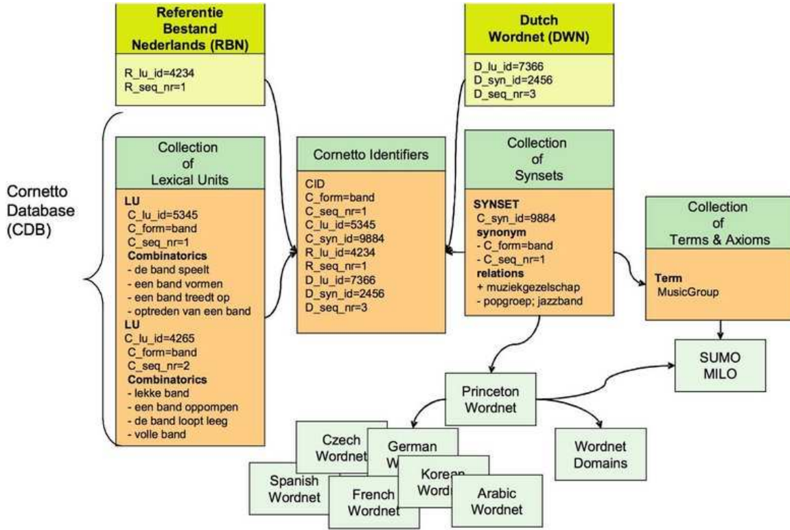
Fig. 1: Data collections in the Cornetto database.
